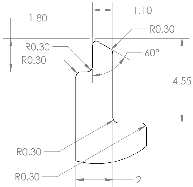
DETAIL B SCALE 8 : 1
